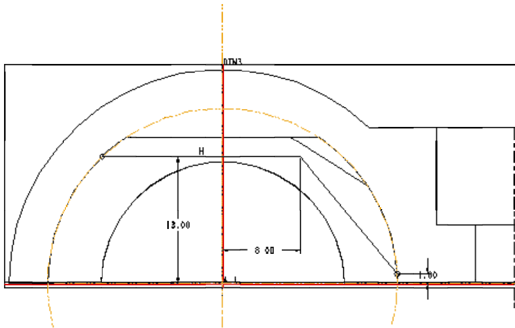
Figure 13: Dimensions of the large reinforcing rib
