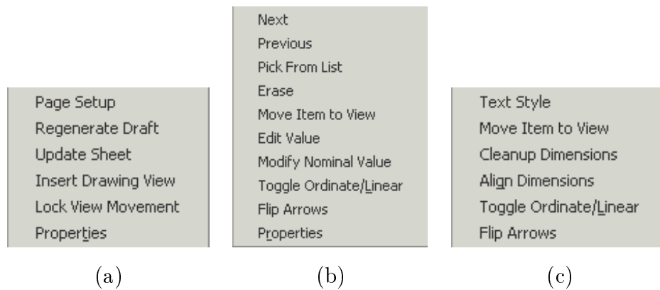
Figure 16: Examples of context sensitive Pull out Menus, (a) On background (b) On selection of 1 dimension (c) Multiple dimension selection
