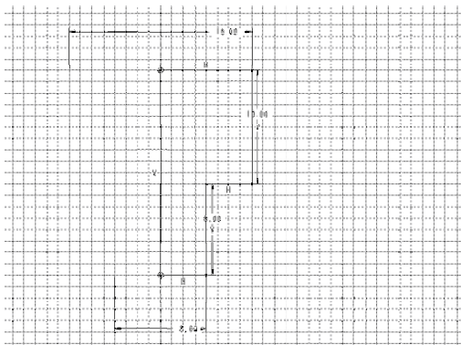
Figure 10: Rough sketch of the sketched hole section.
