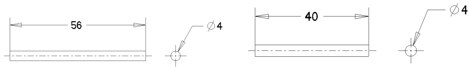
Figure 10: Dimensions of the output and lay shafts
