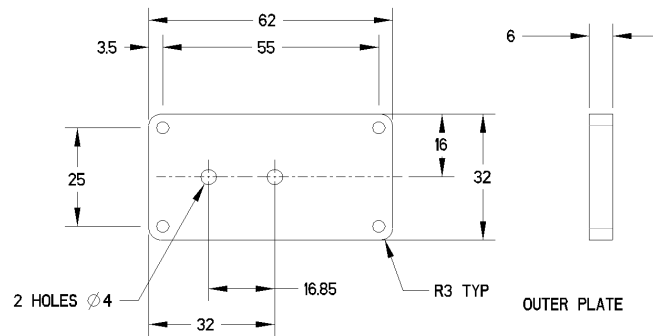
Figure 11: Multi-feature construction (Extrusion - Cut - Drill - Round) used to generate the outer plate
