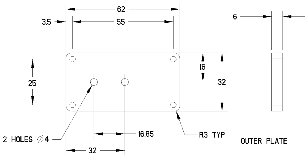
Figure 18: Example of a dimensioned drawing of the Outer_Plate
